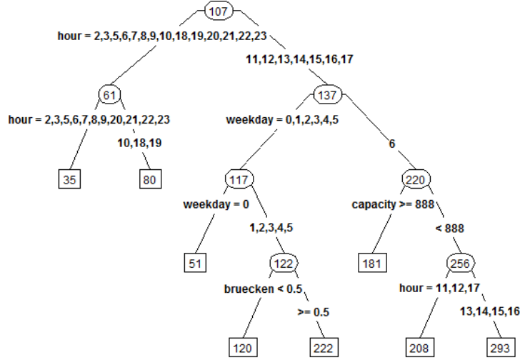
Fig. 4. Sample binary decision tree for Kö Gallerie parking facility (#39)
