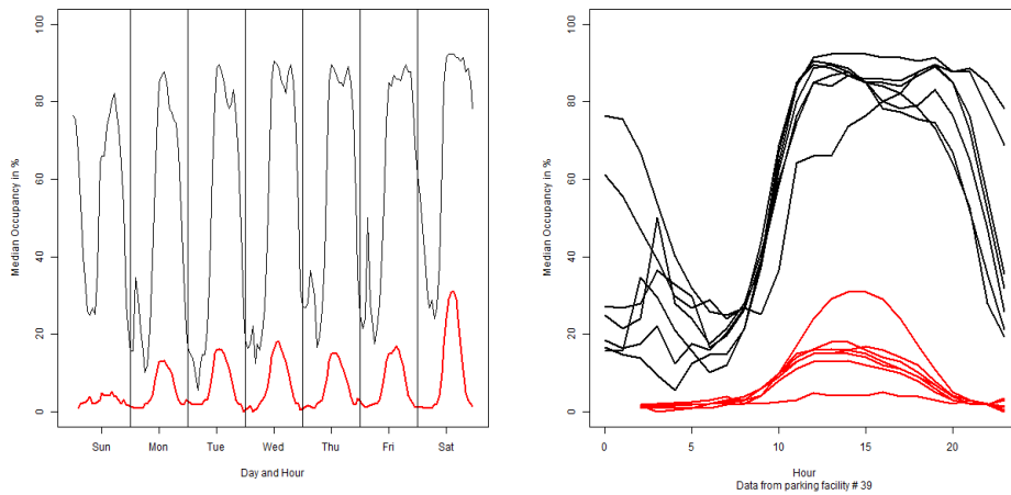
Fig. 3. Periodicity of parking demand with facility-specific temporal patterns (above #3 Kunsthalle (black) and below #39 Kö Gallerie (red))
