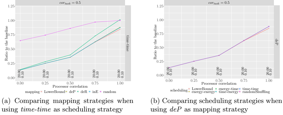
Figure 1: Ratio of energy consumption using different mapping and scheduling strategies under small failure rate, when varying cor_{proc} , with basicWork = 0.3 , \beta_{b/w} = 1 , \mathcal{R}_i = 0.98 and cor_{task} = 0.5 .
