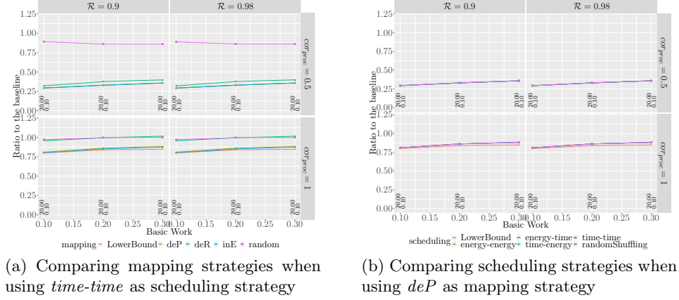
Figure 5: Ratio of energy consumption using different mapping and scheduling strategies when varying basicWork and \mathcal{R}_i , under small failure rate, with \beta_{b/w} = 1 and cor_{task} = 0.5 .
