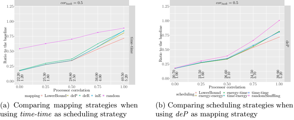
Figure 2: Ratio of energy consumption using different mapping and scheduling strategies under big failure rate, when varying cor_{proc} , with basicWork = 0.3 , \beta_{b/w} = 1 , \mathcal{R}_i = 0.95 and cor_{task} = 0.5 .
