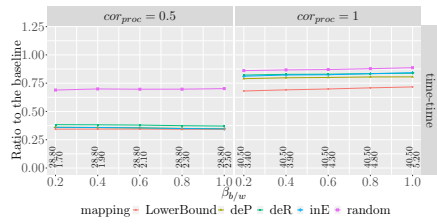
(a) Comparing mapping strategies when using time-time as scheduling strategy
