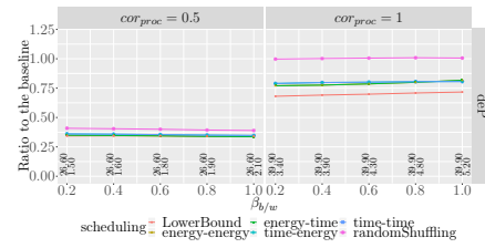
(b) Comparing scheduling strategies when using deP as mapping strategy
