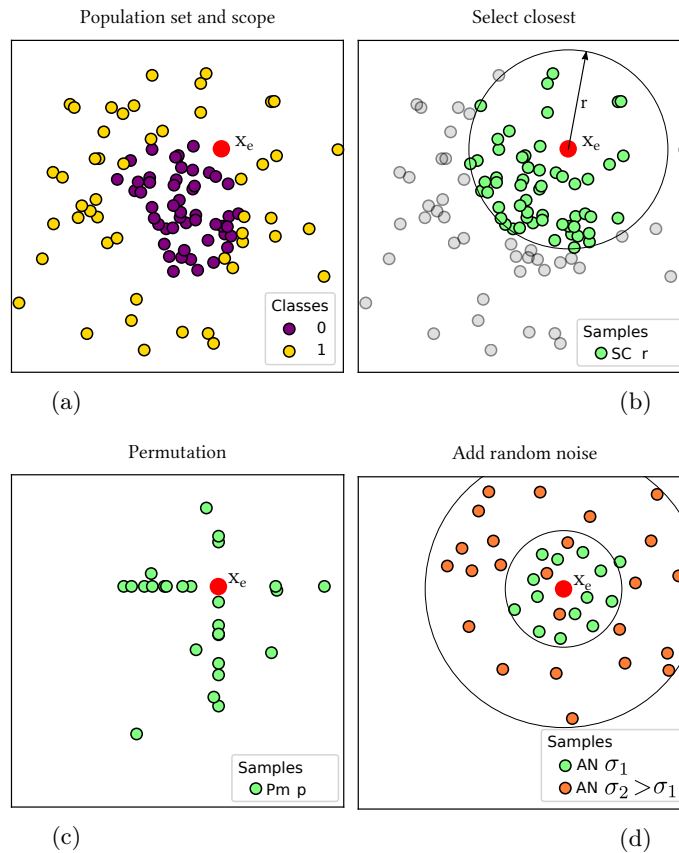
Figure 1: Schematic view of local sampling processes with two dimensional continuous variables. The point of interest of the explanation (or scope) is the red circle x_e . (a) Population set and point of interest for a binary classification problem, classes are depicted with different colors. (b) "Select closest" sampling with threshold r . Samples are inputs of the population set within a circle of size r centered at the point of interest. (c) "Permutation" sampling with probability p . Samples are altered versions of the point of interest with one or two features drawn from the empirical distribution. (d) "Add random Noise" sampling with \sigma_1 and \sigma_2 > \sigma_1 . Samples are noisy versions of the point of interest.
