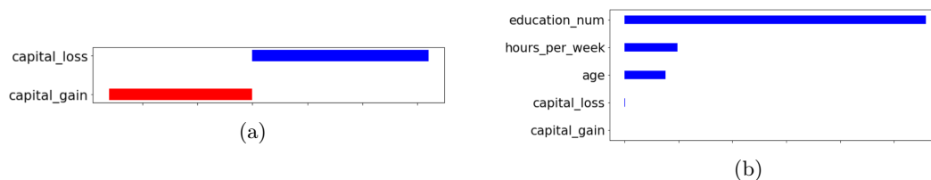
Figure 8: Two LA explanations generated by IBEX for the same adult input predicted as ' < 50k '. The positive values (blue bars) indicate a positive impact of the feature on the output ' < 50k ' and negative values (red bars) indicate a negative impact on the output ' < 50k '. (a) The explanation on the left (generated with realism=1 ) reflects the logic of the ADS, disregarding the actual distribution of the input data. (b) The explanation on the right (generated with realism=3 ) reflects the behaviour of the ADS on real data (based on the distribution of the input data set).
