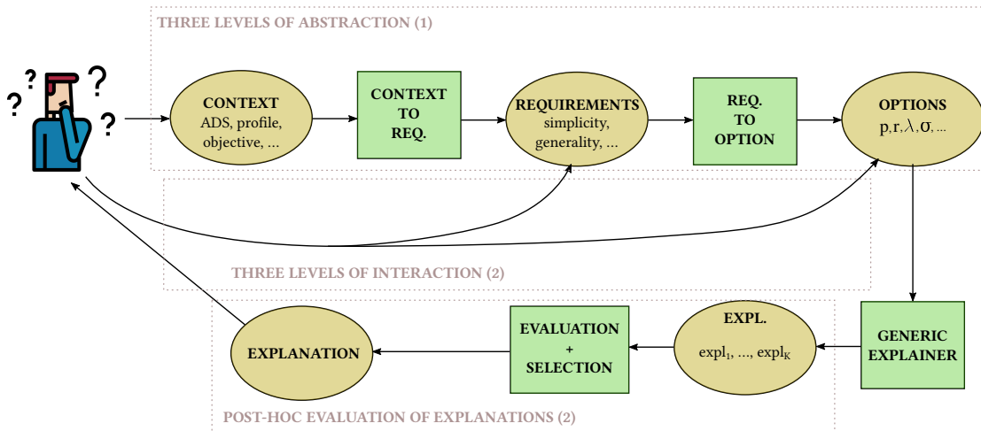
Figure 2: Overview of the approach.
