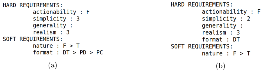
Figure 4: (a) Requirements derived by IBEX from the initial context (G, LU, T) ; (b) Revised requirements based on the user’s request “less simple”.
