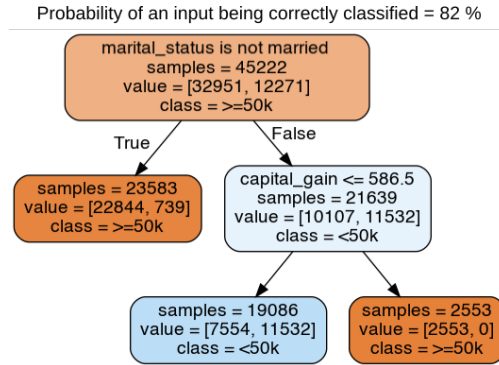
Figure 3: Explanation generated by IBEX for the adult census data set based on the initial context. IBEX has used the following requirements: format=DT, simplicity=3, actionability=F, nature=T, realism=3
