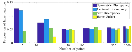
(b) Proportion of false negative in 3D, \varepsilon = 0.05
