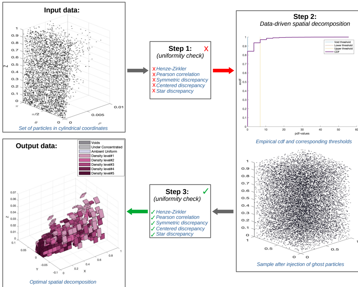
Figure 13: Half-pipe case with transformation of data method. Processing elements and post-processing results for an initial sample \mathbf{X} with n = 3820 fluid particles.
