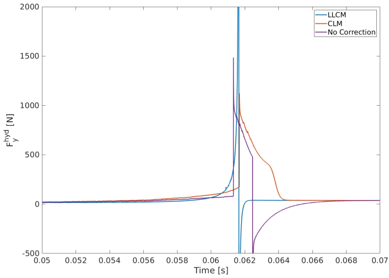
FIGURE 11 Evolution of the total hydrodynamic force acting along the y-direction. Simulations without lubrication correction, with LLMC and CLM are performed using h = 1/40 grid resolution and \mathcal{AR} = 2 . LLMC and CLM parameters are \epsilon_{\text{lub}} = 2/h and \epsilon_{\Delta x} = 0.06 .
