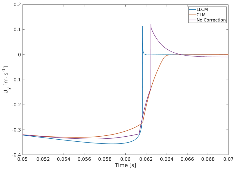
FIGURE 12 Evolution of the particle vertical velocity. Simulations without lubrication correction, with LLMC and CLM are performed using h = 1/40 grid resolution and \mathcal{AR} = 2 . LLMC and CLM parameters are \epsilon_{\text{lub}} = 2/h and \epsilon_{\Delta x} = 0.06 .
