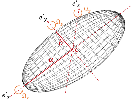
FIGURE 2 Representation of the particle with surface mesh in coordinate system (e'_x, e'_y, e'_z) .
