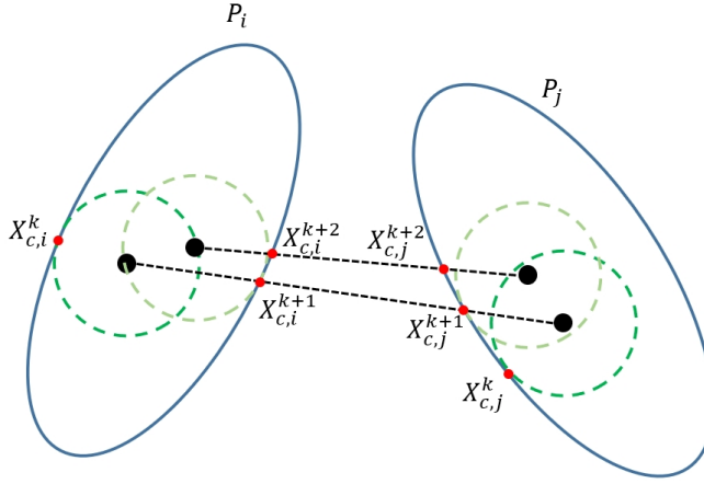
FIGURE 3 Two-dimensional sketch of the iterative method of Lin et al. [25] used to compute the distance between two ellipsoids.
