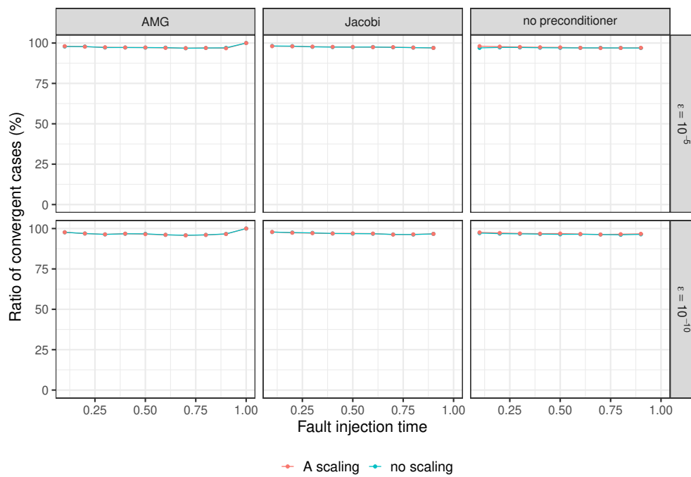
Figure 1.5: Impact of the bit-flip injection time in the preconditioner application on PCG convergence success.
