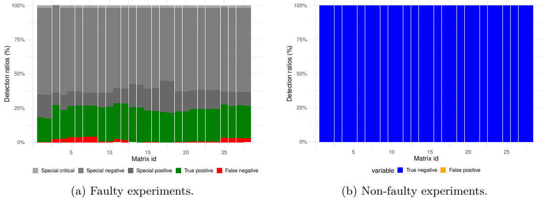
Figure 4.2: Ratio of missed errors (a) and false-positives (b) with the non-optimal thresholds \tau = 2.30e-7 for the experiments with \varepsilon = 1e-10 and a Jacobi preconditioner.
