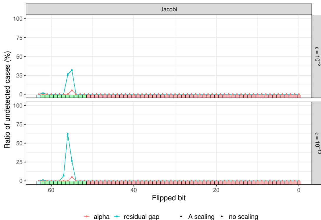
Figure 4.5: Detection performance of the residual gap and \alpha -based methodologies for soft errors in the preconditioner calculation.
