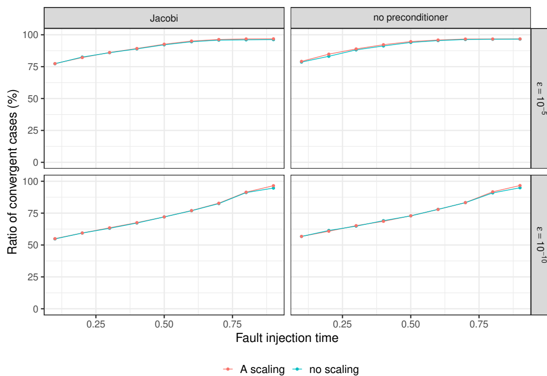
Figure 3.5: Impact of the bit-flip injection time (as a proportion of the number of iterations with respect to the non-faulty execution) in the matrix-vector product on PCG convergence success.
