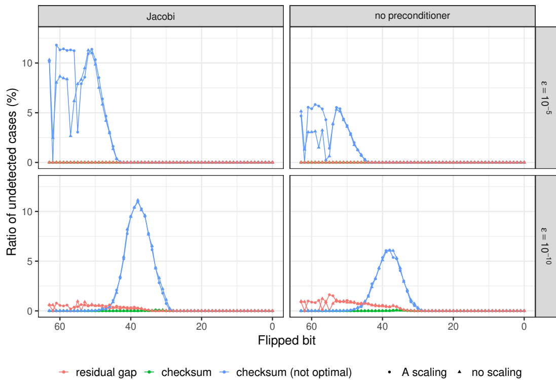
Figure 4.4: Detection performance of gap deviation and checksum-based methodologies for soft errors in the matrix-vector calculation.
