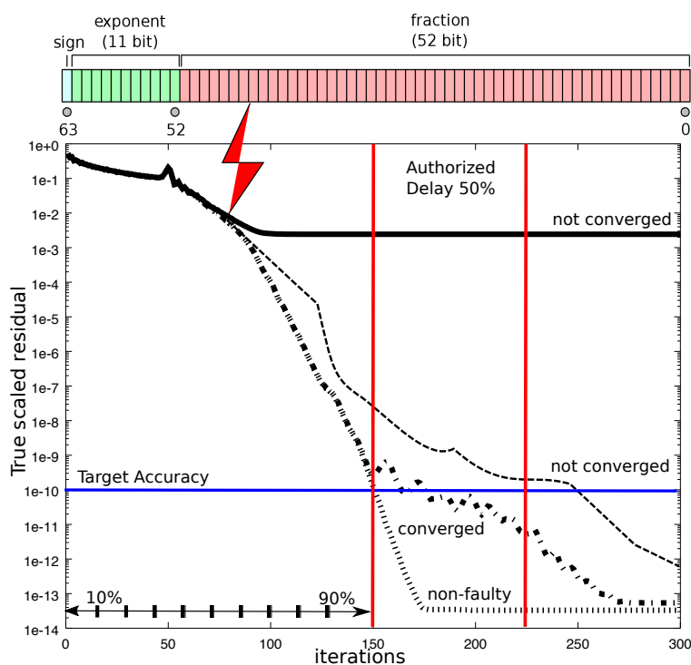
Figure 3.2: The error is injected in the input vector at any entry, any bit and at any time in the iterative process for either the matrix-vector product or the preconditioner calculation.
