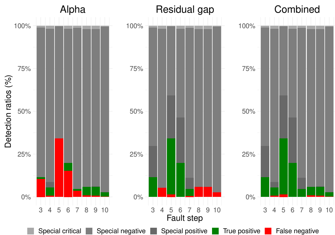
Figure 4.6: Comparison of the detection success of the alpha and residual gap based methodologies, and their combination for bit-flips in all possible steps of PCG. The set PCG runs used for this experiment is different from the other experiments, but was created using the same methodology described in Section 3.2: the only differences are the total number of runs and the possible locations for the bit-flip.
