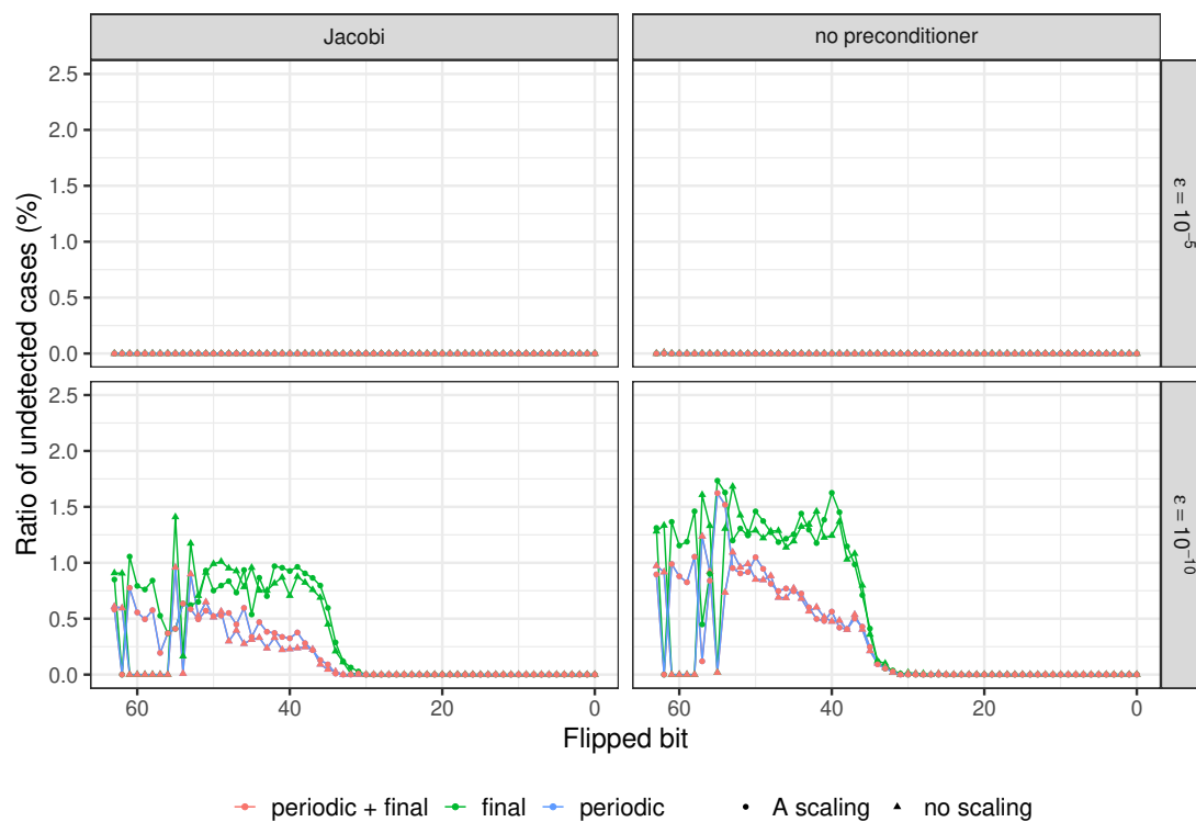
Figure 4.3: Detection performance of the three policies based on the residual gap criterion.
