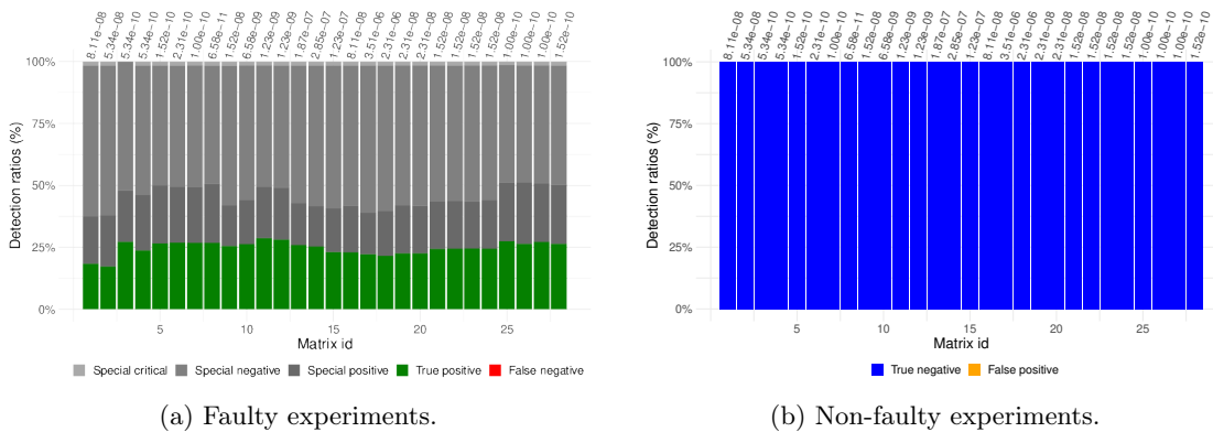
Figure 4.1: Ratio of missed errors (a) and false-positives (b) with the optimal thresholds \tau (top of the bars) for the experiments with \varepsilon = 1e-10 and a Jacobi preconditioner.
