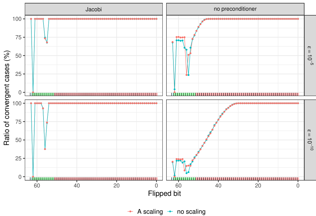
Figure 3.6: Impact of the index of the flipped bit in the preconditioner application on PCG convergence success.
