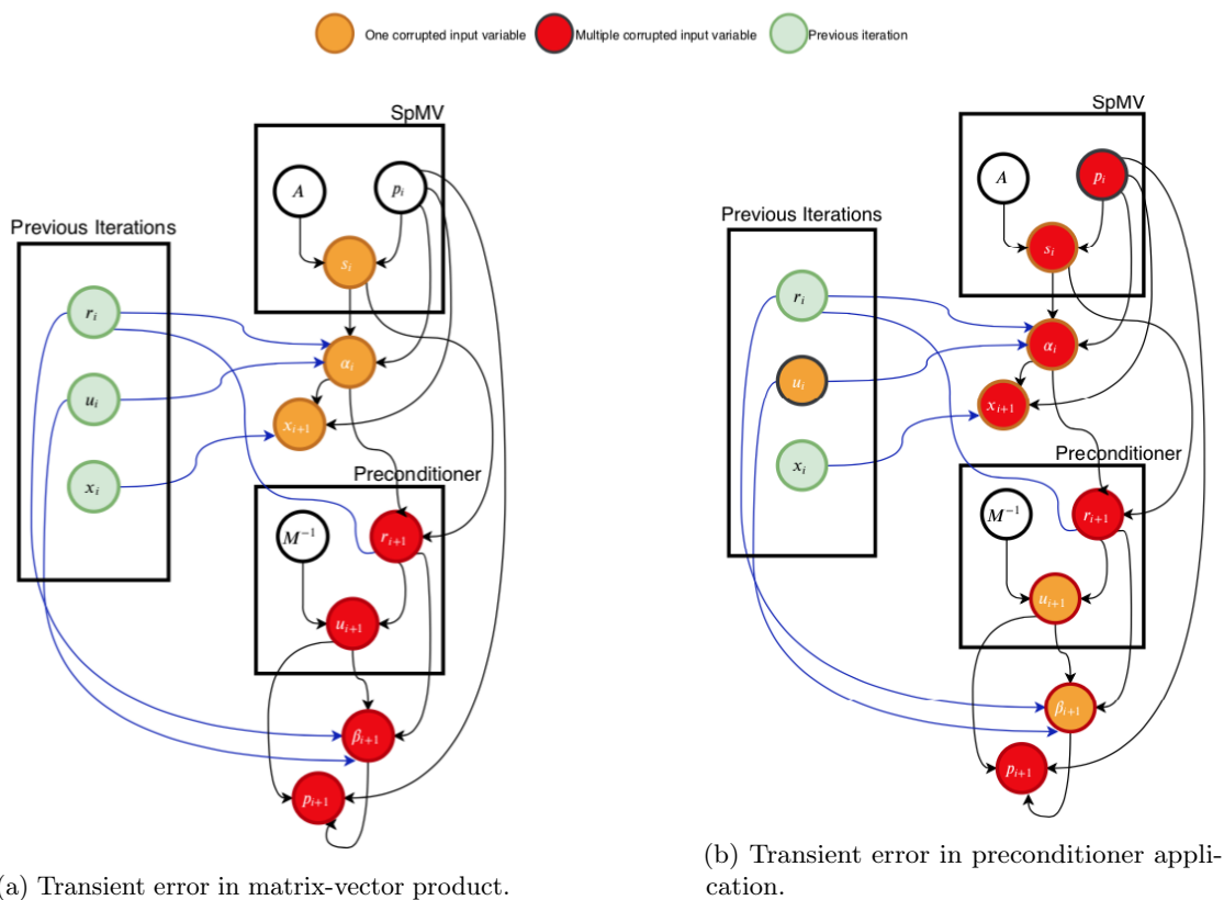
Figure 3.1: Propagation of transient errors in the PCG algorithm.
