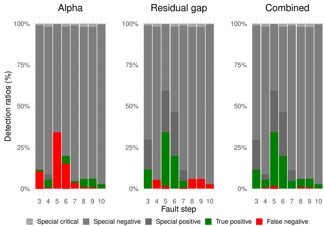
Figure 14: Comparison of the detection success of the alpha and residual gap based methodologies, and their combination for bit-flips in all possible steps of PCG. The set PCG runs used for this experiment is different from the other experiments, but was created using the same methodology described in Section 3.2: the only differences are the total number of runs and the possible locations for the bit-flip.
