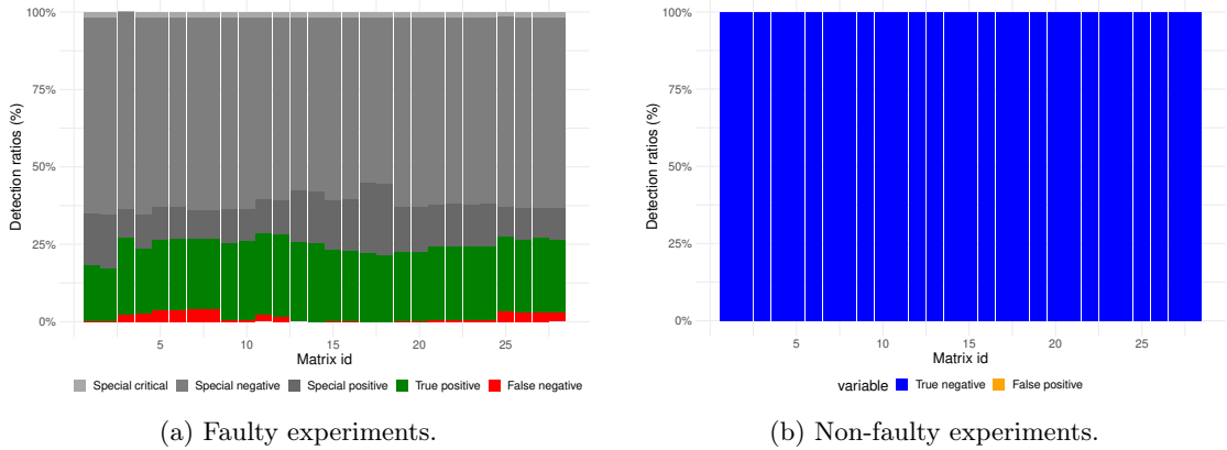
Figure 10: Ratio of missed errors (a) and false-positives (b) with the non-optimal thresholds \tau = 2.30e-7 for the experiments with \varepsilon = 1e-10 and a Jacobi preconditioner.
