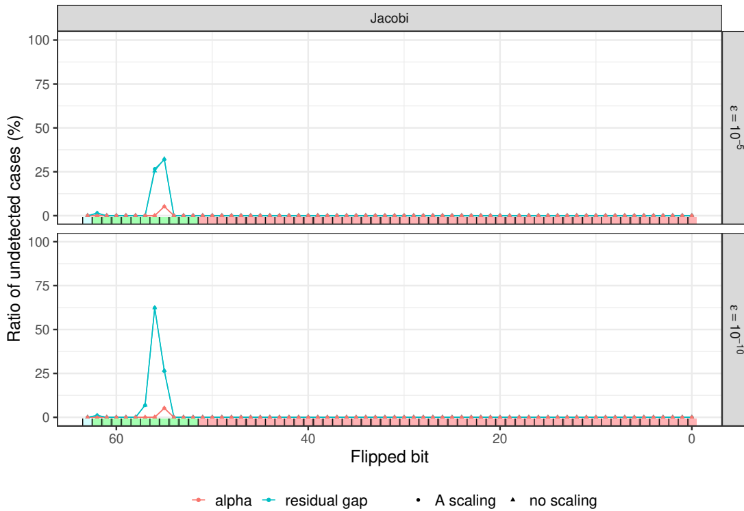
Figure 13: Detection performance of the residual gap and \alpha -based methodologies for soft errors in the preconditioner calculation.
