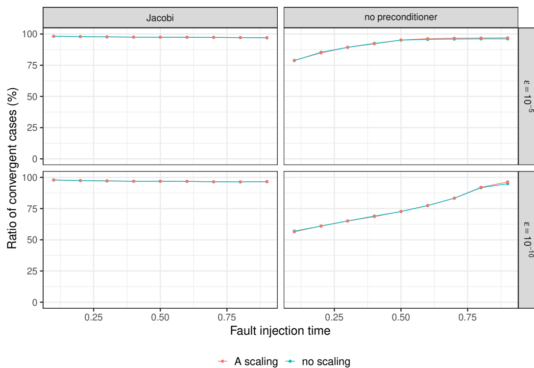
Figure 8: Impact of the bit-flip injection time in the preconditioner application on PCG convergence success.
