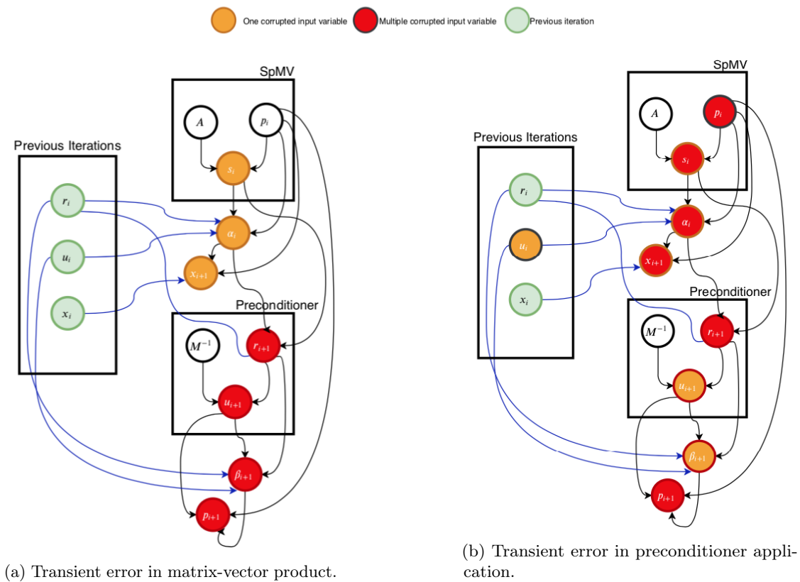
Figure 2: Propagation of transient errors in the PCG algorithm.
