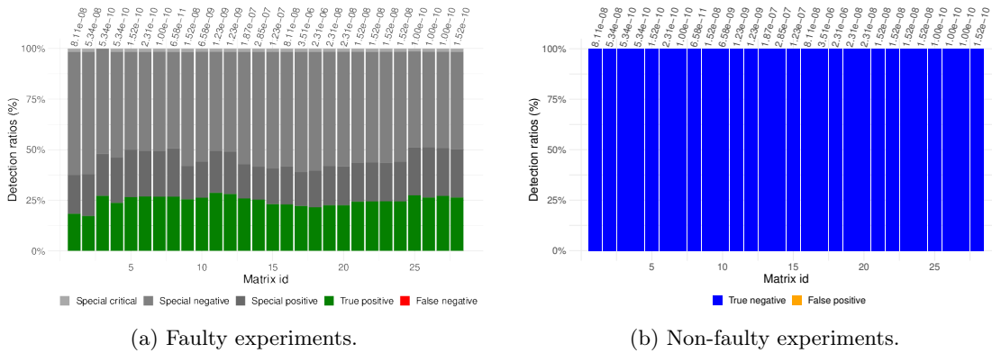
Figure 9: Ratio of missed errors (a) and false-positives (b) with the optimal thresholds \tau (top of the bars) for the experiments with \epsilon = 1e-10 and a Jacobi preconditioner.
