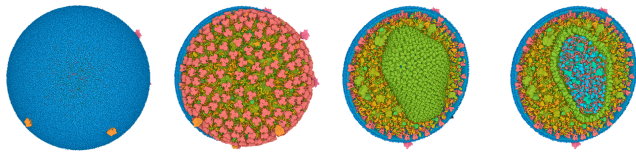
Fig. 1. The organization of models from structural biology can be complex and it is often impossible to convey its architecture using just a single view and cutting settings. Here, we consecutively open up a model of an HIV particle to show its several levels, each communicating a different spatial subpart of the virus.
