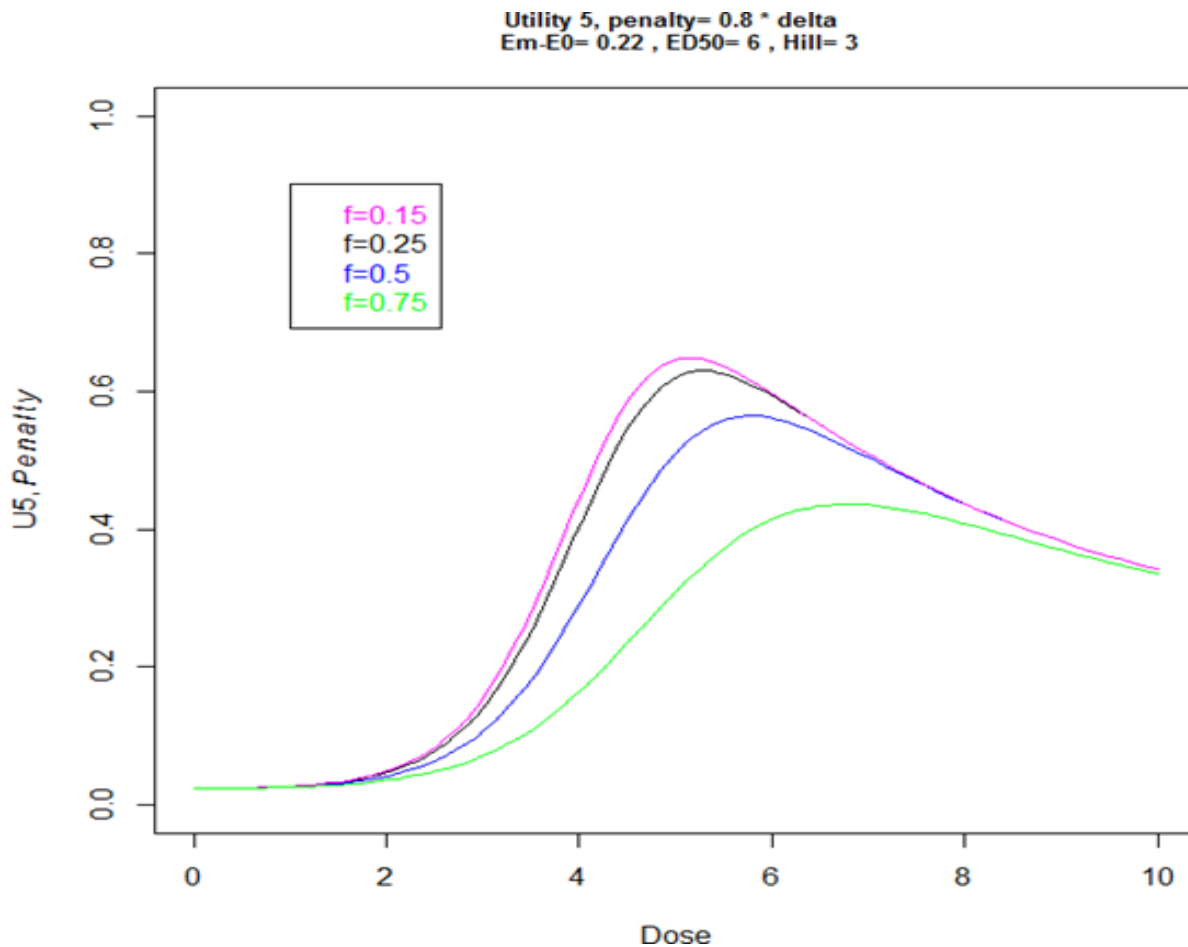
Figure 5: Theoretical utilities as a function of the dose and f
