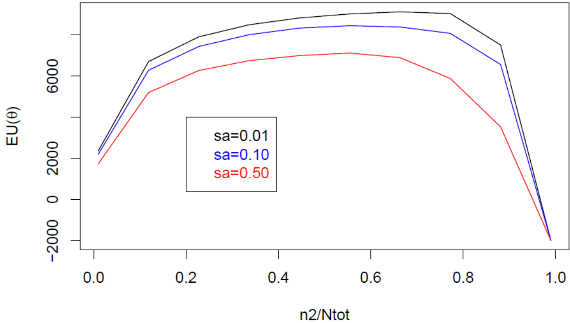
Figure 3: Utility as a function of phase II sample size and safety sa
