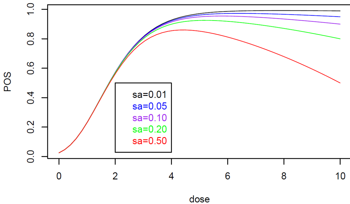
Figure 2: PoS by dose for various values of the safety parameter
