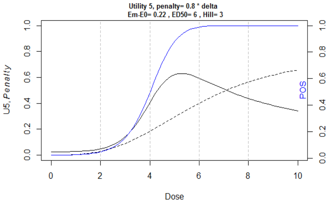
Figure 4: Theoretical curves for U5, Sigmoid scenario
