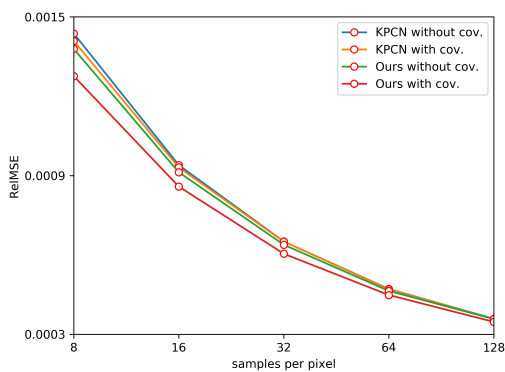
Fig. 10 RelMSE Comparison between our method (with light transport covariance), our method (without light transport covariance), KPCN (without light transport covariance) and KPCN (with light transport covariance) over varying sample count.
