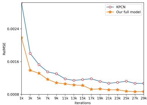
Fig. 8 Comparison of RelMSE as a function of training iterations of our method and KPCN. Our method is always better than KPCN at any iteration.
