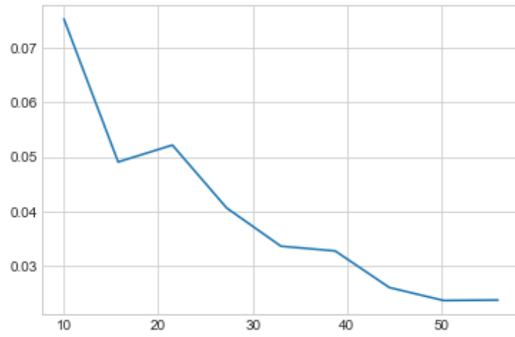
Figure 24: Relative Difference between ALAP and the Lower Bound, GPU case, for different sizes of n .
