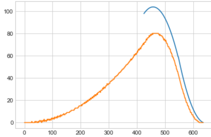
Figure 13: Overall number of GEMM tasks f_{\#}(t) , ( n = 40 ), GPU case
