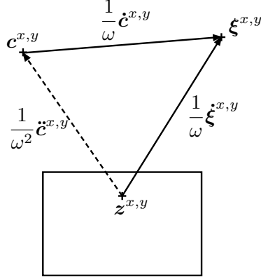
Figure 48.8: The speed of the CoM, c , points towards the Capture Point, \xi , while the speed of this Capture Point points away from the CoP, z . The combination of these two first-order dynamics gives the acceleration, \ddot{c} , pushing the CoM away from the CoP.
