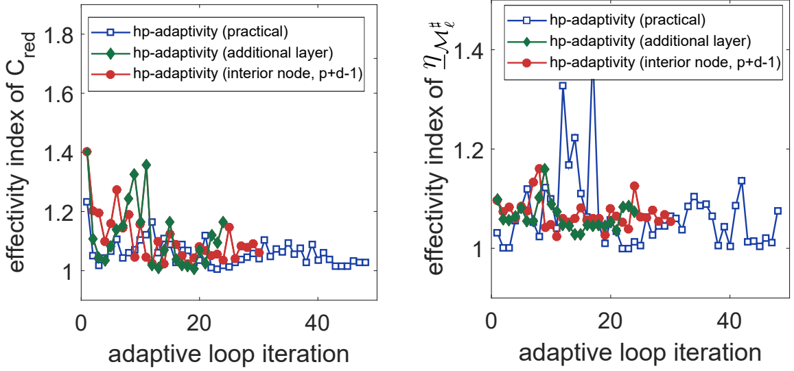
Figure 5: Effectivity index for the error reduction factor estimate C_{\ell,\text{red}} of Theorem 6.1 given by (10.1) (left); effectivity index for the discrete lower bound \underline{\eta}_{\mathcal{M}_\ell^\#} of (4.16) given by (10.2) (right). The “additional layer” hp strategy of Section 4.3.2, the “interior node, p + d - 1 ” hp strategy of Section 4.3.3, and the “practical” hp strategy from [24, Figure 15]. Exact algebraic solver.
