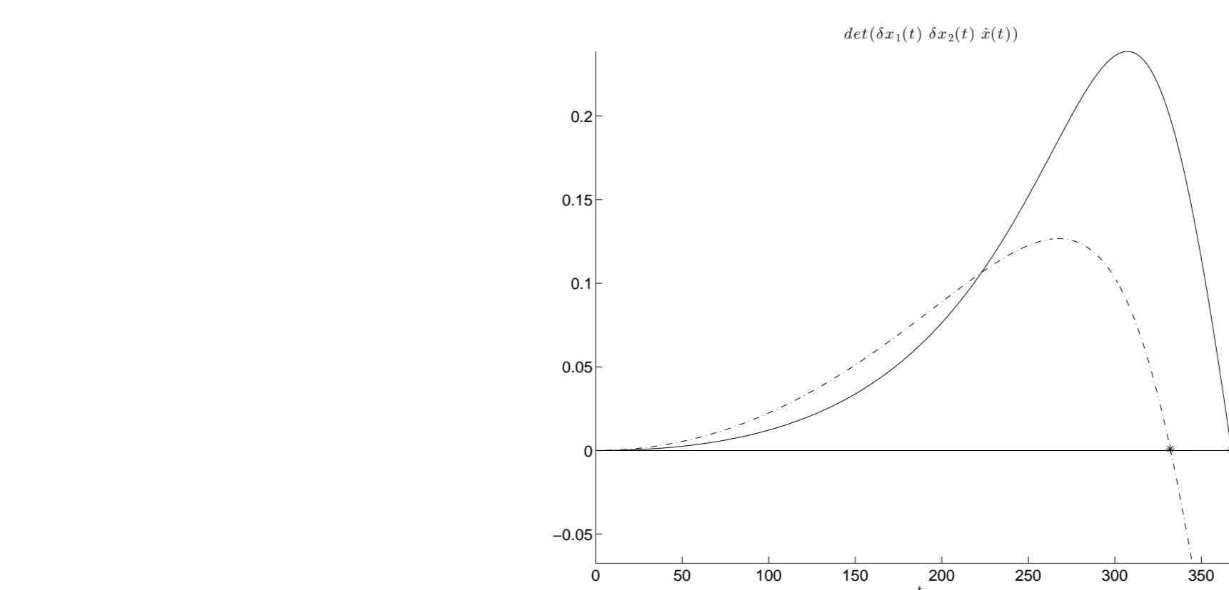
Rank test condition (4) for the perturbed and unperturbed problem.
