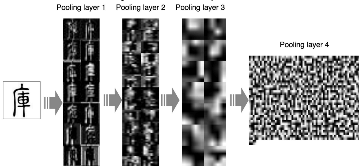
Figure 12. Visual expression of feature map in max pooling layer.
