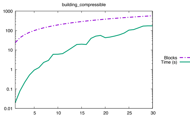
Figure 15: Number of blocks and CPU time for the structural analysis of the building model with compressible air.
