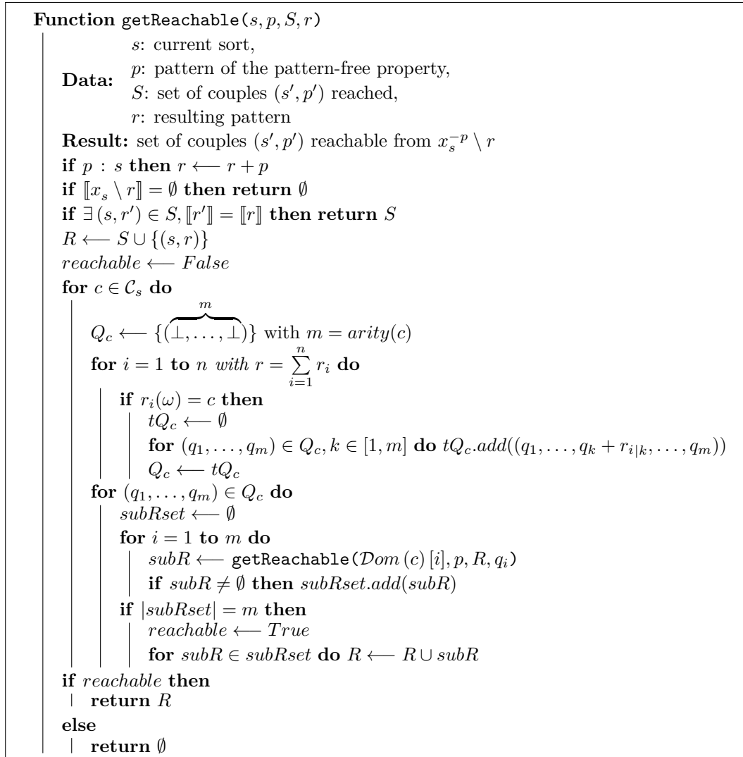
■ Figure 1 Compute deep semantics of quasi-additive terms as a union of ground semantics.
