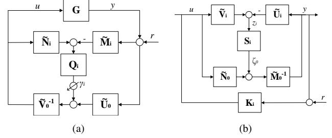
Fig. 2. (a) YK parameterization for controller reconfiguration and (b) Dual YK parameterization for CL identification.
