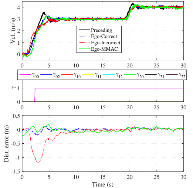
Fig. 13. Experimental results MMAC CACC. Homogeneous string of two cycabs.
