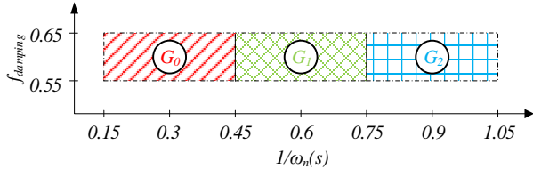
Fig. 5. Uncertainty range string stable for pairs (\mathbf{G}_0, \mathbf{K}_0) , (\mathbf{G}_1, \mathbf{K}_1) and (\mathbf{G}_2, \mathbf{K}_2) .
