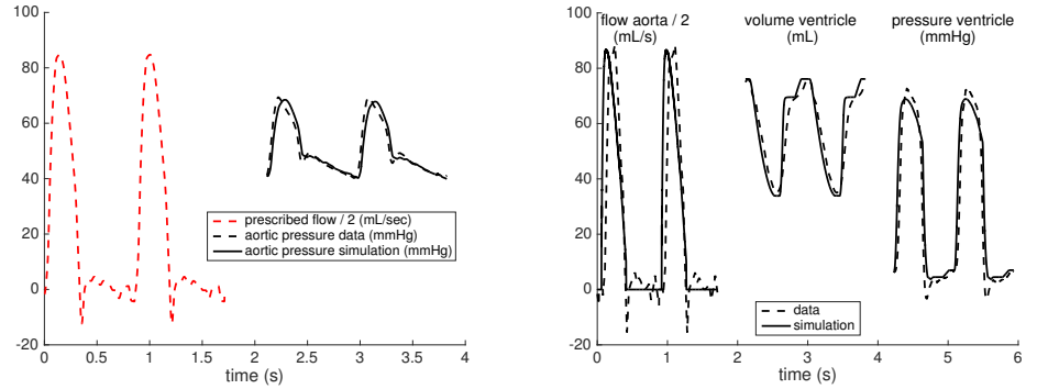
Fig 4. Model calibrations. Calibration of the Windkessel model (left), and of the heart model with prescribed level of preload (right) at rest. For visualization purposes, the aortic flow was downscaled by a factor of 2.
