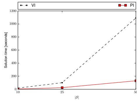
Fig. 1. Performance of PI against VI.
