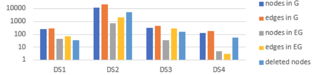
Figure 5: Impact of the graph abstraction algorithms.
