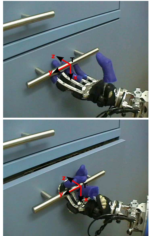
Fig. 6. The task frame is set to the handle. The task is specified as a velocity reference along negative Z axis. A power grasp is performed.
