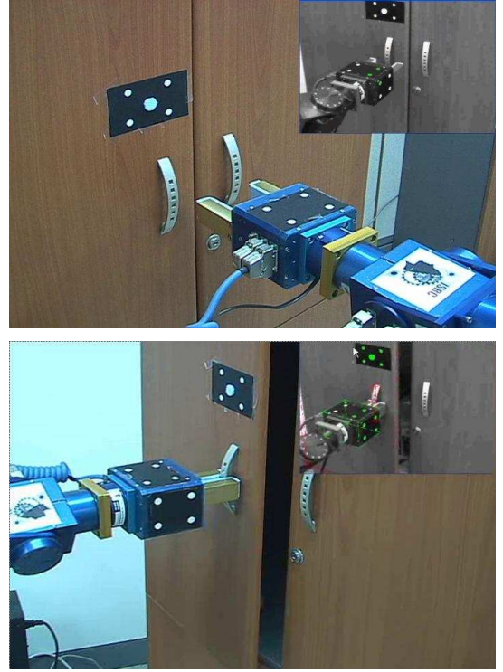
Fig. 5. The mobile manipulator at ISRC opening a door by means of force and vision combination
