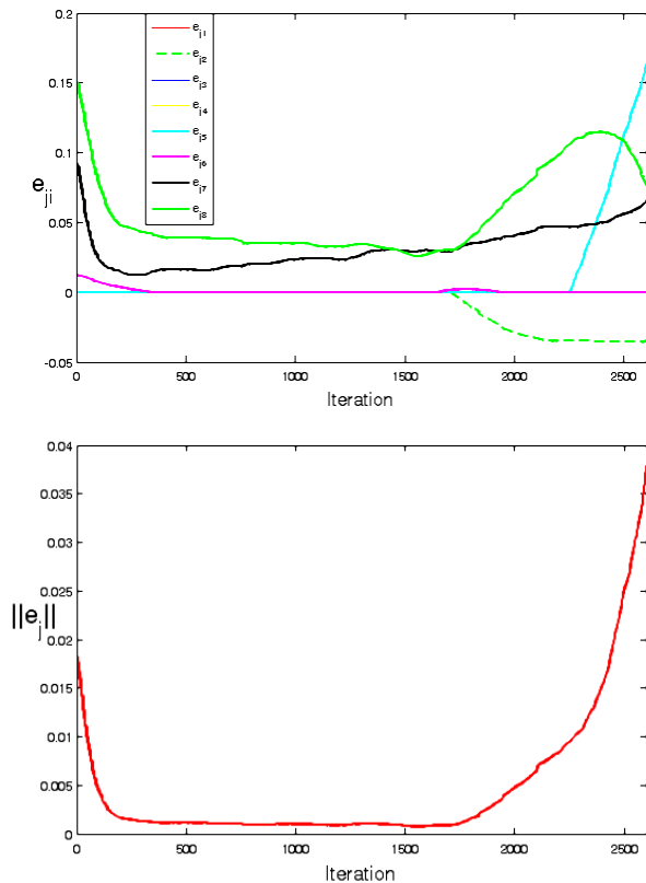
Fig. 8. Effects of the secondary task. Top: cost for each joint. Down: norm of the cost vector.
