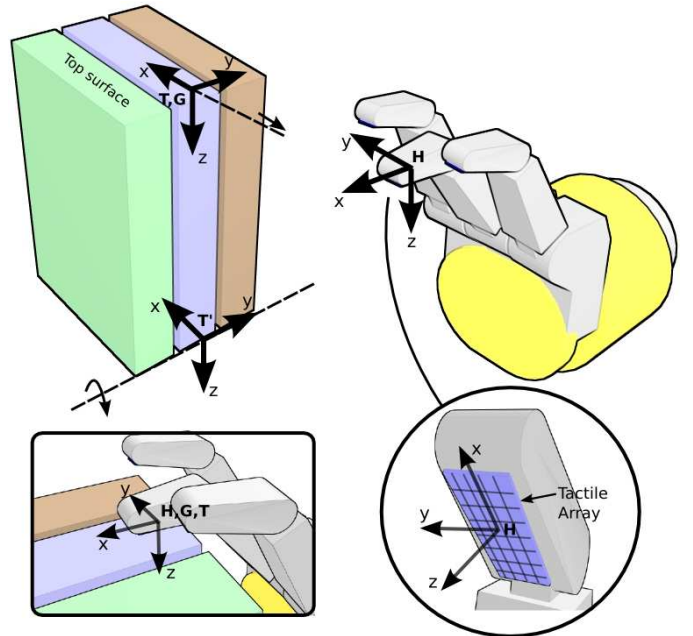
Fig. 2. Frames involved in the book grasping task. The tactile array is used to estimate the relationship between the hand and the grasp frame, {}^H\mathbf{M}_G .
