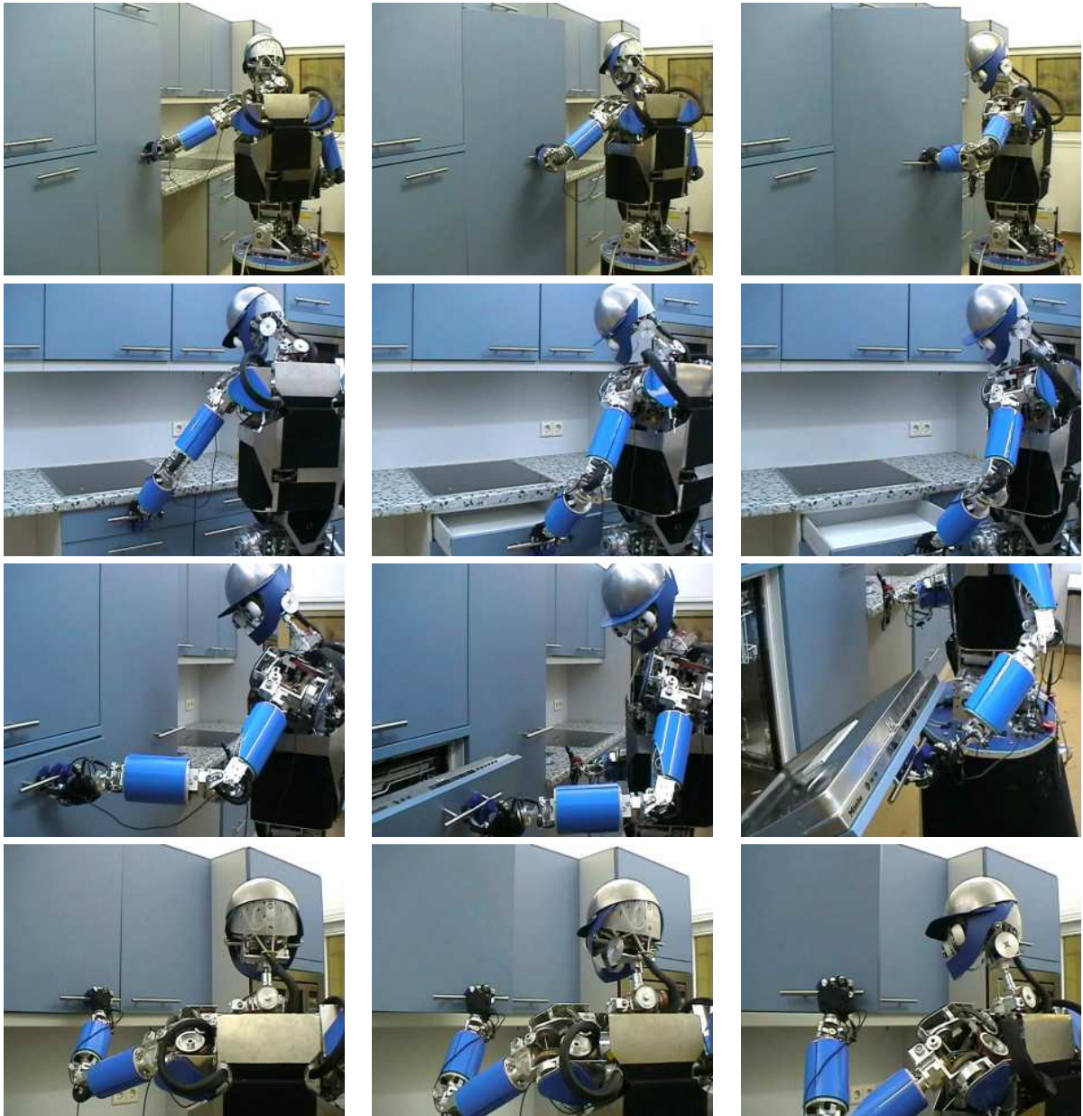
Fig. 7. The Armar-III robot interacting with the kitchen furniture: fridge, drawers, dishwasher and cupboards
