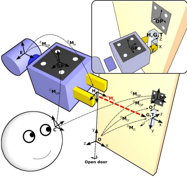
Fig. 4. The vision task is to align hand frame \mathcal{H} with the grasp frame \mathcal{G} .
