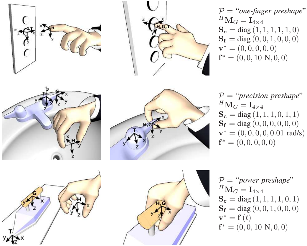
Fig. 1. Some task examples supported by the task-oriented grasping framework. First: pushing a button, with a force reference. Second: turning on a tap, with a velocity reference. Third: ironing task, with a velocity and force reference. T , H and G are, respectively, the task , hand and grasp frame.
