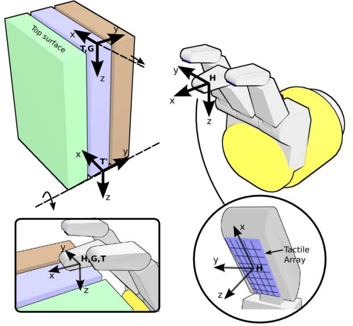
Fig. 2. Frames involved in the book grasping task. The tactile array is used to estimate the relationship between the hand and the grasp frame, {}^H\widehat{\mathbf{M}}_G .
