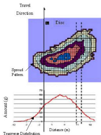
Fig. 1. Spread pattern (spatial distribution) and transverse distribution
