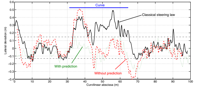
Fig. 9. Lateral deviation during path #1 following
