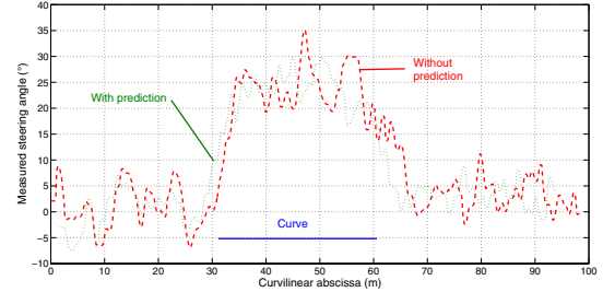
Fig. 8. Steering angle (path #1 following) with and without prediction
