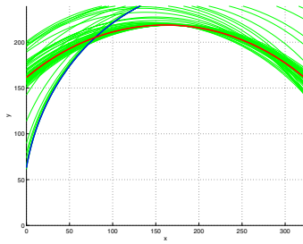
Fig. 7. Trajectories in the image plane of line projection with an hypercatadioptric camera
