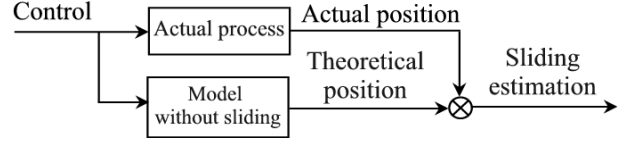
Fig. 6. Sliding detection
