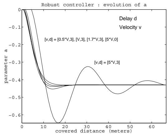
Figure 6: Influence of the data flow latency
