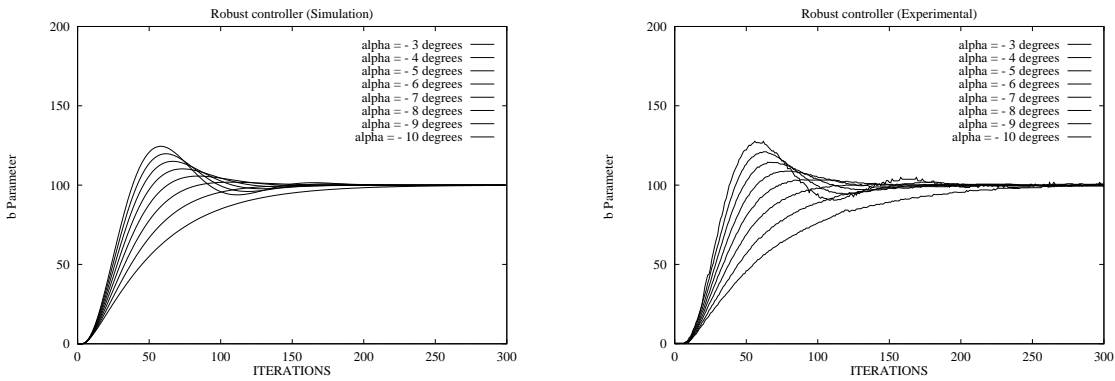
Fig. 4. Robust control approach: b Output behaviour ( \alpha from -3 to -10 degrees)
