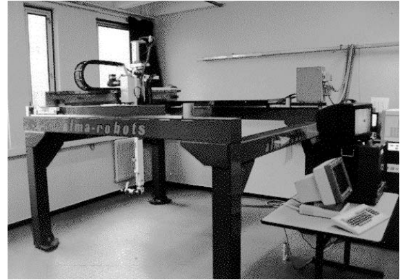
Figure 6 Overview of the robotic platform.
