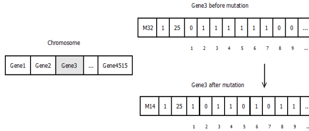
Fig. 3: Example of a mutation operation
