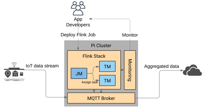
Fig. 4. Demonstration setup
