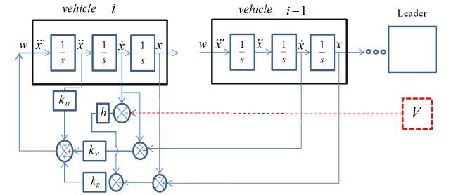
Fig. 5. Control scheme of the i -th vehicle
