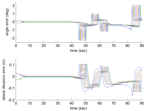
Fig. 9. Lateral angle and distance errors(part A,B).
