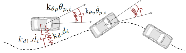
Fig. 4. Lateral Platoon Model
