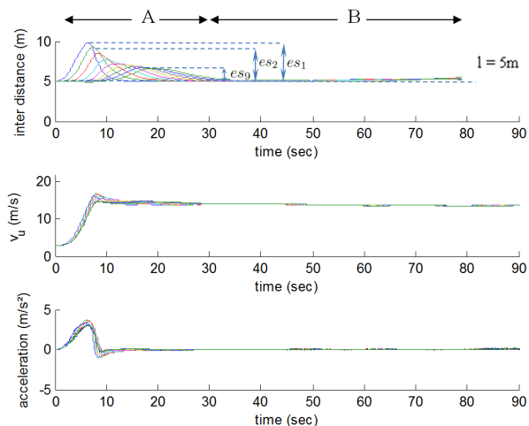
Fig. 8. inter-vehicle distances and vehicle's velocities(part A,B).
