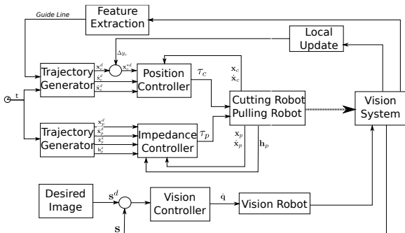
Fig. 4. Global Control Scheme
