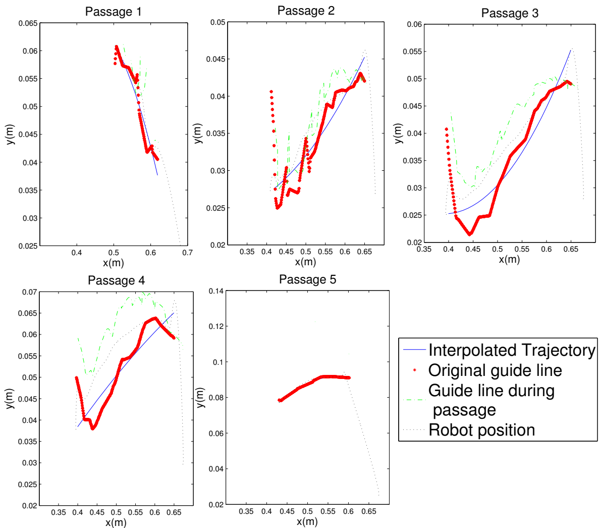
Fig. 7. Robot Trajectory modified by local updates
