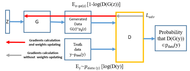
Figure 2. Functioning schema of adversarial neural network.
