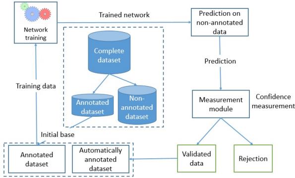
Figure 1. Functioning schema of a semi-automatic learning algorithm.
