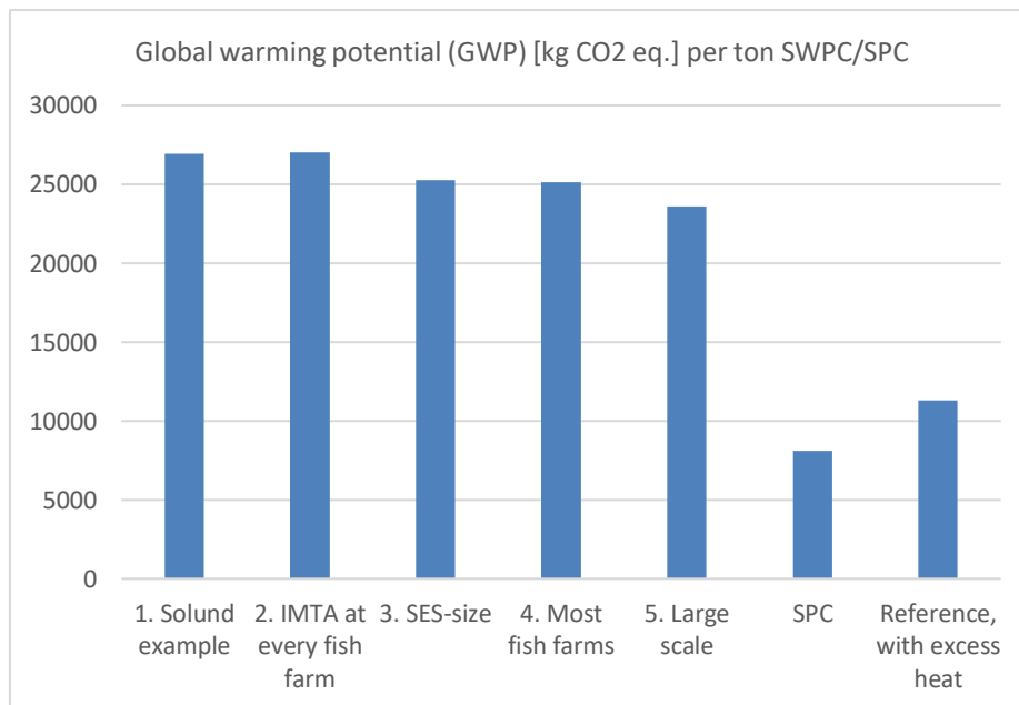
Figure 2. Global warming potential (GWP) for the five different cultivation scenarios, SPC production and an alternative version of scenario 1.
