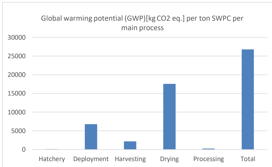
Figure 3. Global warming potential (GWP) for the reference scenario (Solund example), shown per main step of the value chain.
