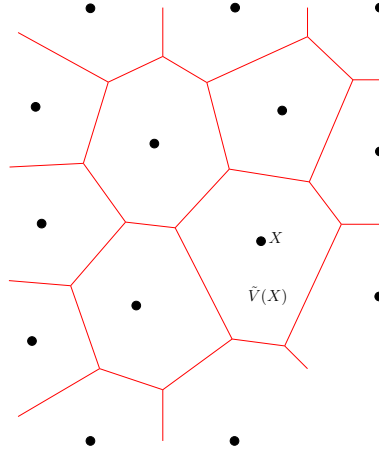
Figure 6.1: Voronoi cell
