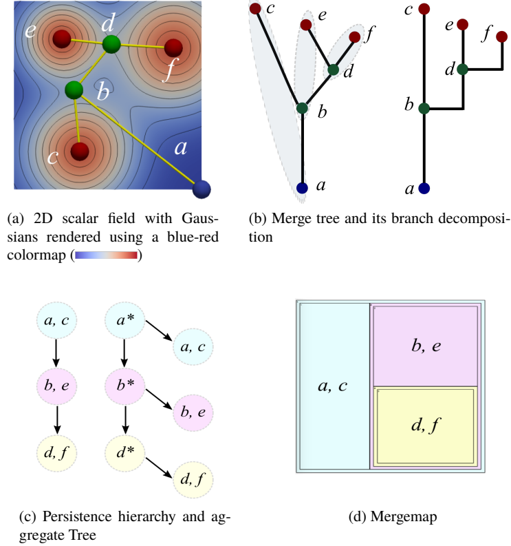
Fig. 3: Constructing a mergemap for a scalar field
