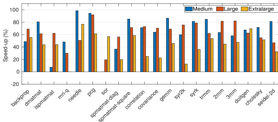
Figure 6. Maximum speed-up with unlimited invocations against Apollo without multi-versioning (Magerit: 20 threads/cores)
