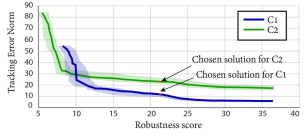
Fig. 3: Median Pareto front (thick line) and associated IQR (colored region) computed by NSGA-II in 20 runs with a population of 100 individuals and 300 generations for the controllers C1 (blue) and C2 (green).
