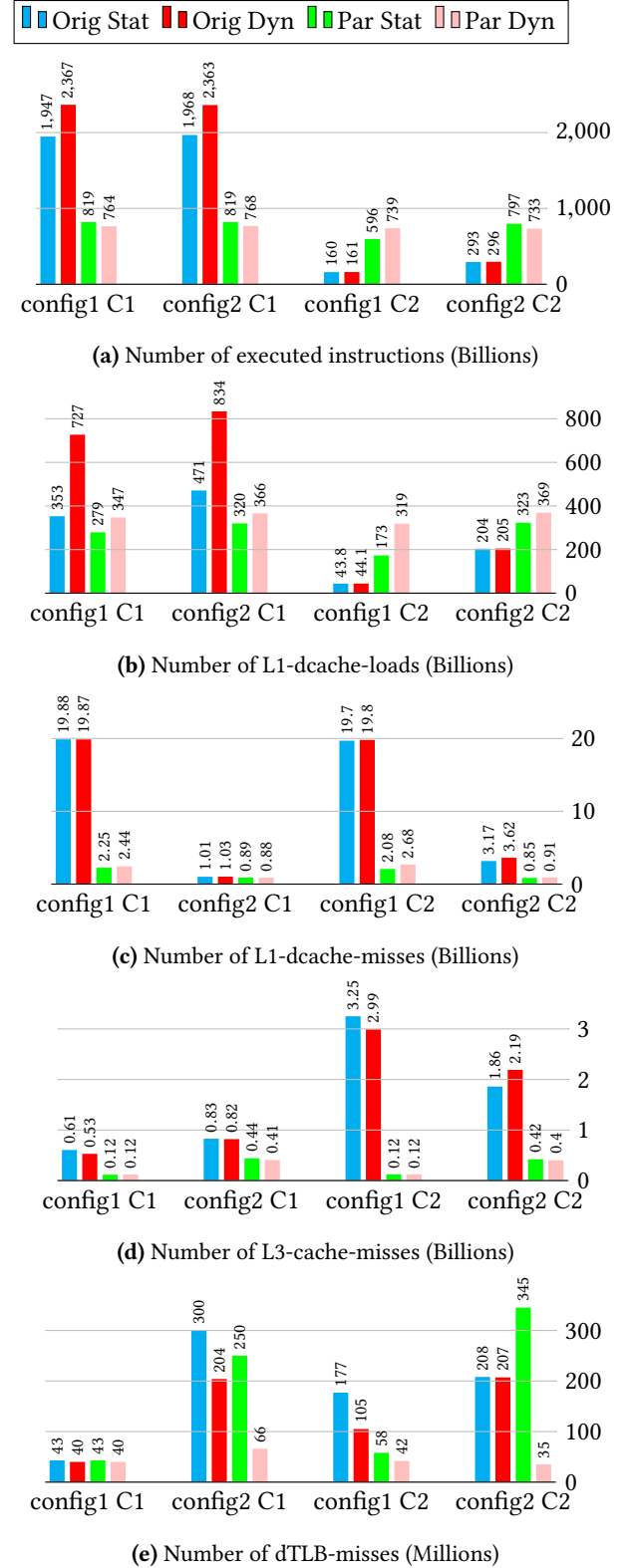
Figure 8. Performance counters for static and dynamic allocations, on config1 and config2, for C1 and C2 codes
