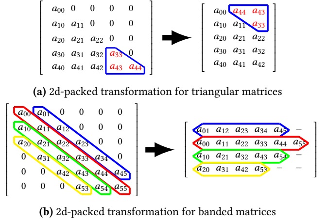
Figure 1. New data structures for different sparse matrices
