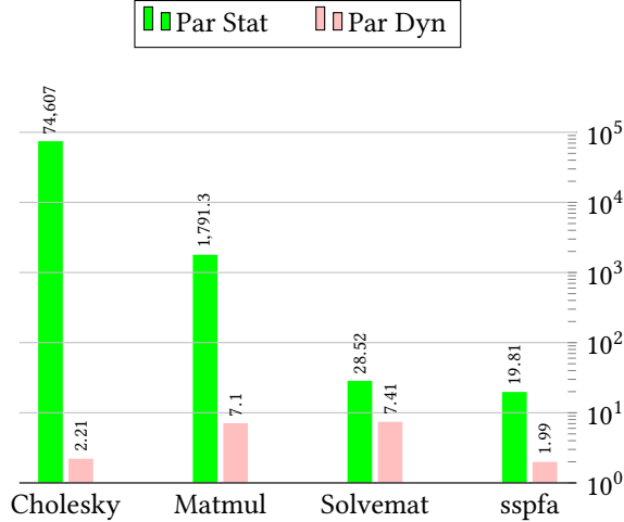
Figure 10. Number of vectorized instructions (Millions, logscale) for static and dynamic allocations on config1 for the 2d-packed benchmarks
