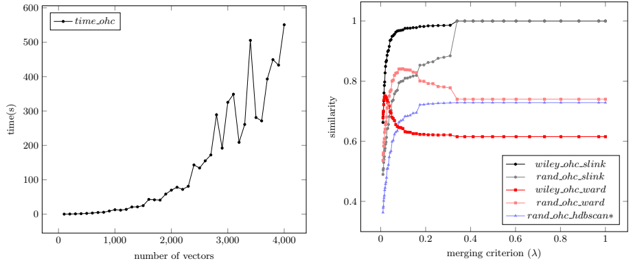
(a) Execution time according to the number of vectors. (b) Similarity between hierarchical structures according to the merging criterion.
