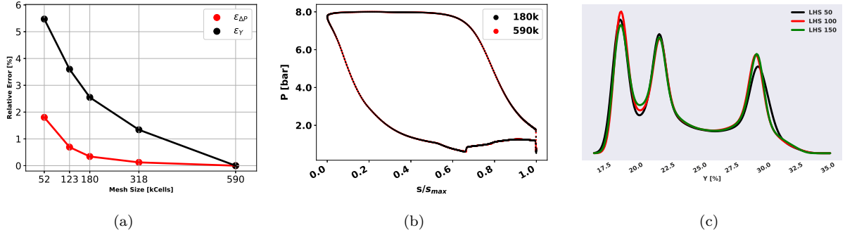
Figure 5: RANS Grid Analysis on the baseline configuration. (a) \Delta P and Y Relative Error, (b) Pressure Distribution comparison between 180k and 590k cells meshes, (c) Y PDF obtained on the 180k cells mesh, for different LHS size.
