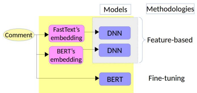
Fig. 1. Proposed methodology
